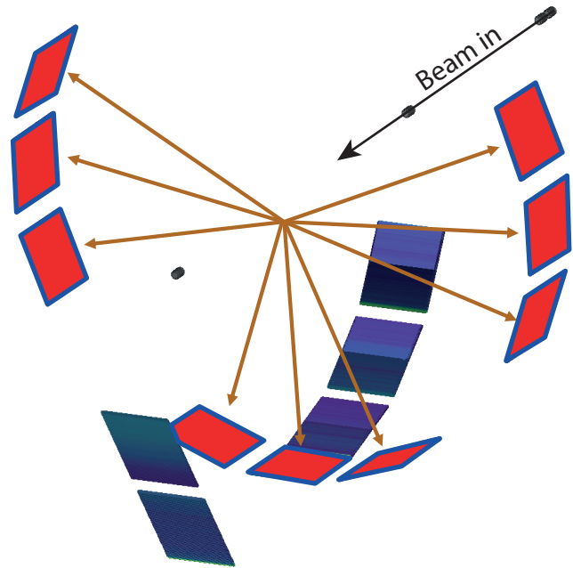
'Transverse' scattering geometry
