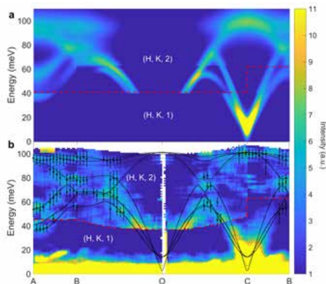
Inelastic neutron scattering data of Mn_3Sn over the full Brillouin zone at 4K, and calculated magnon spectra using a linear spin wave theory. Black solid and dashed lines on the data shows the calculated magnon dispersion relation. Error bars indicate one sigma of the magnon energy fitted by the data.
