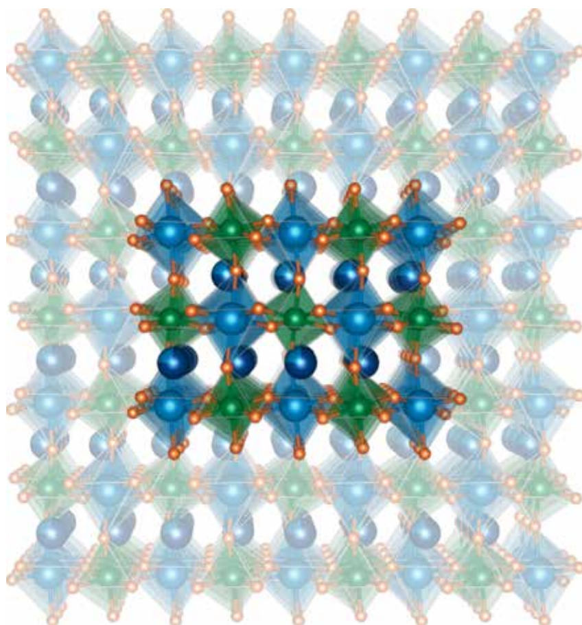
Crystal structure of the Na-rich double perovskite, Na 1.5 La 1.5 TeO 6
