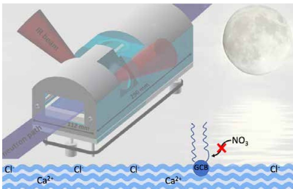
Applying a novel experimental set-up that combines simultaneous interrogation of floating one-molecule thin films by infra-red (IR) spectroscopy and neutron reflectometry demonstrated that night-time oxidation by \text{NO}_3^\cdot cannot fully remove a galactocerebroside (GCB) monolayer from the sea surface on atmospherically relevant timescales, leaving its saturated tail at the interface.
