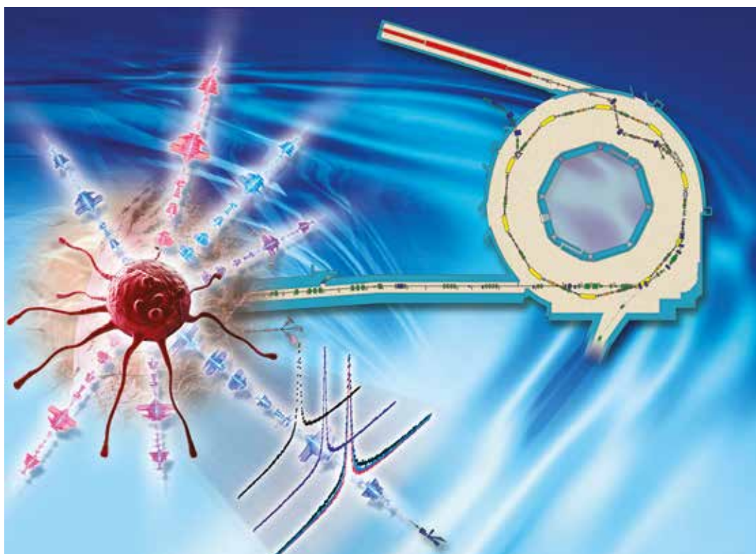
Reproduced from M. P. M. Marques et al. "Intracellular water – an overlooked drug target? Cisplatin impact in cancer cells probed by neutrons" Phys. Chem. Chem. Phys. 19 (2017), 2702-2713 DOI: 10.1039/C6CP05198G with permission from the PCCP Owner Societies.
