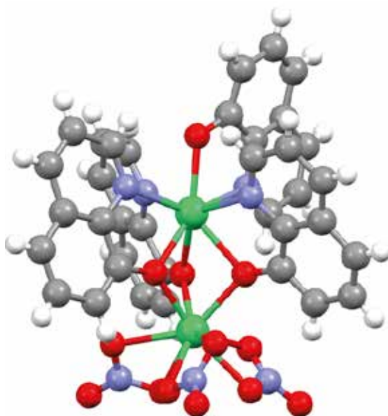
Asymmetric dimetallic lanthanide molecules were studied with EPR and INS spectroscopies to unravel the fine magnetic structure due to the exchange interaction
